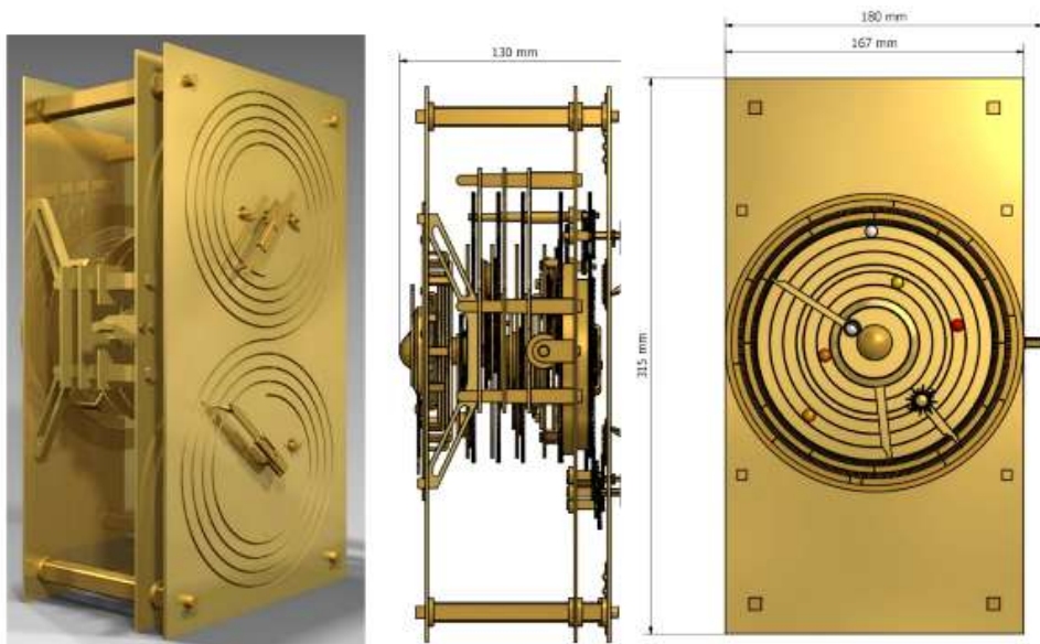
The planetarium clock we built with the University of Mexico Sonora and the Relojes Olvera III Generacion monumental clock Mexican Company.
