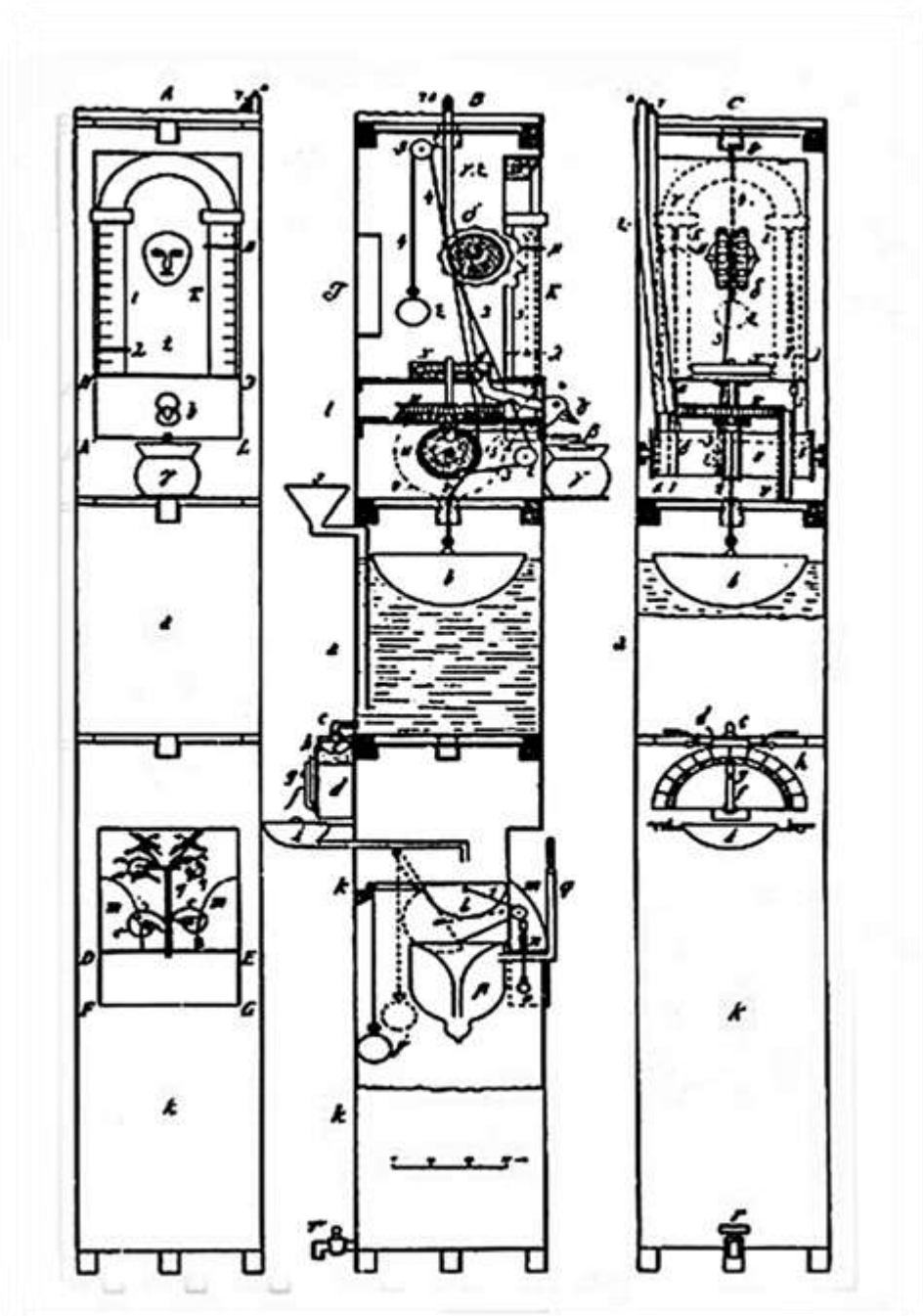
Archimedes clock. The Antikythera Mechanism probably works in a similar way with weight sn counter weights regulated by a float and water. E. Stamatis, Archimedes Works, ed. TEE
