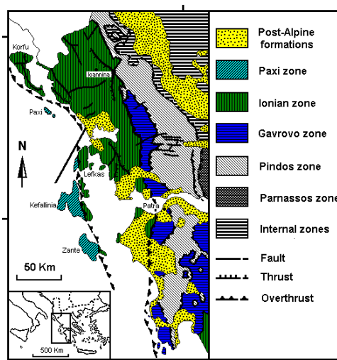
Figure 1 – Geotectonic map of Western Greece
