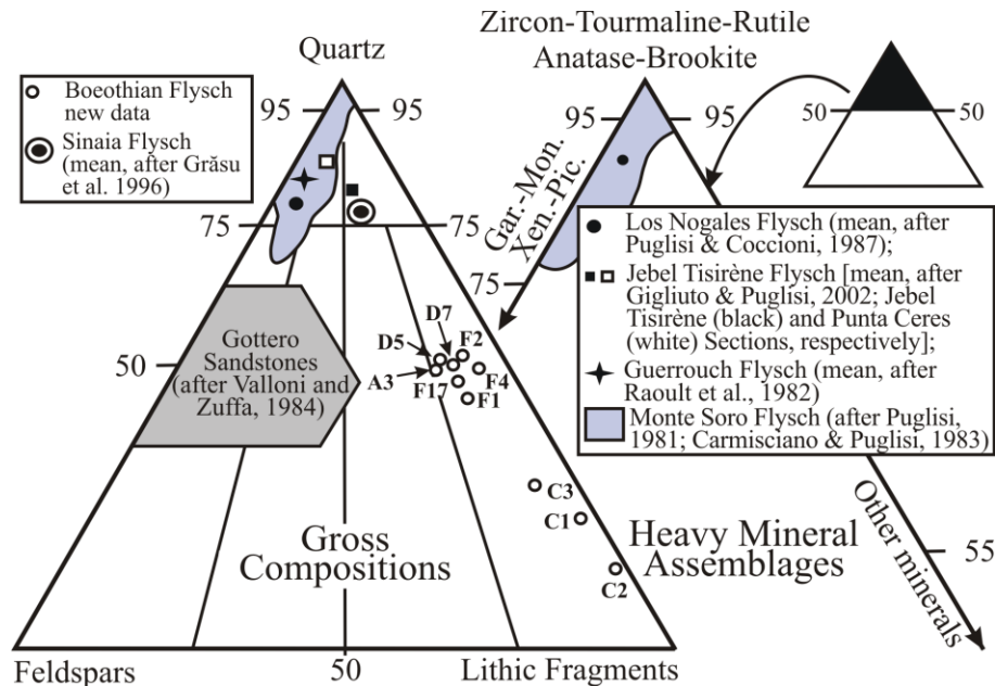
Fig. 5. Quartz-Feldspar-Lithic Fragment and Heavy Mineral Assemblage ternary plots showing the gross co-mposition characterizing the sandstones of the Early Cretaceous Maghrebian flysch (i.e. Los Nogales, Tisirène, Guerrouch and Monte Soro Flysch), northern Apennines (Gottero Sandstones) and eastern Carpathians (Sinaia Flysch). The data of the heavy mineral assemblages available in literature only regard two Early Cretaceous Maghrebian flysch (i.e. Los Nogales and Monte Soro Flysch; Puglisi, 1981; 1987; Puglisi and Coccioni, 1987). Heavy Mineral Assemblage abbreviations: Gar= garnet, Mon= monazite, Xen= xenotime and Pic= picotite).
