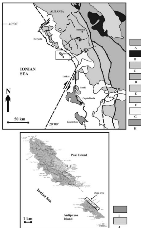
Fig. 1: On top, simplified geologic map of Western Greece (Karakitsios & Rigakis 2007). A. Pelagonian domain; B. Ophiolites; C. Mesohellenic molasse; D. Pindos zone; E. Gavrovo-Tripolis zone; F. Ionian zone; G. Neogene – Quaternary (post-Alpine sediments); H. Preapulian zone. On bottom, geological map of Paxi and Antipaxos Islands (adapted from Perry et al. 1960). I. Early Eocene - Early Miocene; J. Late Cretaceous - Middle Eocene.
