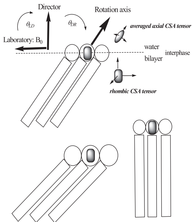
FIGURE 2 Overall view of the entire model system revealing the basic geometrical parameters such as the angle \vartheta_{DR} between the director and the rotation axis. (Lower panels) Impact of the dimensions of the headgroup on the collective tilt and on the bilayer order: lower left, voluminous headgroup (e.g., phosphatidylcholine); lower right, small headgroup (e.g., phosphatidylethanolamine).
