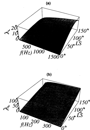
FIG. 7. (a) This three-dimensional plot shows how the opening angle \lambda_L of \hat{\mathbf{L}} changes with frequency (from 10 Hz up to the frequency of the last stable orbit) for various \tilde{\mathbf{L}}\mathbf{S} angles, for two representative binaries: (a) a 1.4M_\odot , 1.4M_\odot NS-NS binary with one of the stars maximally rotating, S_i = M_i^2 ; (b) a 10M_\odot , 1.4M_\odot BH-NS binary with the black hole maximally rotating.
