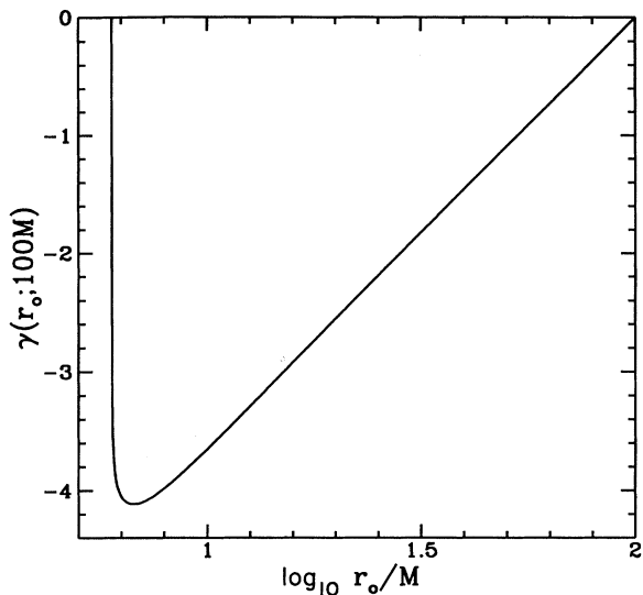
FIG. 2. A plot of \gamma(r_0, r_i) , as defined in Eq. (1.5), for r_i = 100M , as a function of \log_{10} r_0/M . The curve may be continued, both to the left and to the right, using the analytical estimates (1.6)–(1.8). For example, \gamma(1000M; 100M) \simeq 3.6392 . The function \gamma(r_0; r_i) has a minimum at r_0 = r_c \simeq 6.6792M , and grows to plus infinity when r_0 \rightarrow 6M . Horizontal lines intersect the curve at two distinct points ( r_0 = r_1 and r_0 = r_2 ) for which the eccentricity is equal, \varepsilon(r_1) = \varepsilon(r_2) .
