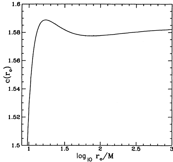
FIG. 1. A plot of c(r_0) , as defined in Eq. (1.2), as a function of \log_{10} r_0/M . Shown is the range 10 \lesssim r_0/M < 1000 , in which c(r_0) has the most interesting behavior. For r_0/M > 1000 , c(r_0) is well approximated by Eq. (1.3), and approaches the value 19/12 \simeq 1.5833 as r_0 tends to infinity. The function c(r_0) changes sign at r_0 = r_c \simeq 6.6792M , and approaches minus infinity when r_0 \rightarrow 6M , in a way well described by Eq. (1.4).
