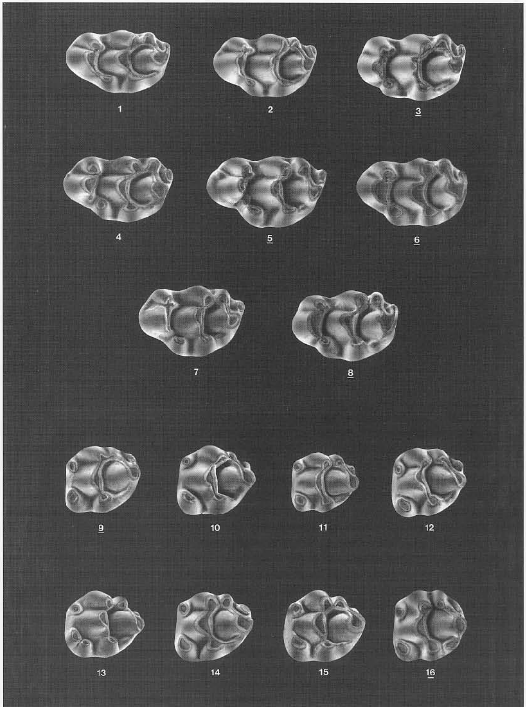
PLATE 2 Apodemus sp. I from Düzyayla. Figs. 1-8: M1, figs. 9-16: M2. The teeth have been arranged in a sequence according to the development of the t7. The frequency distribution of the various morphotypes is given in (text)Figure 3. The M2 of figure 13 is the only specimen with a t1 bis.
