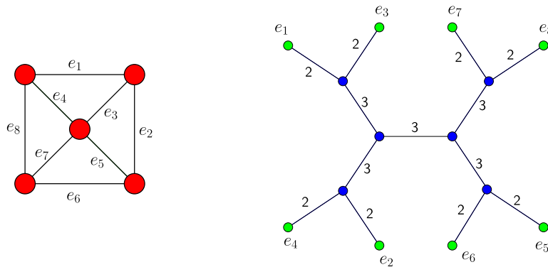
Fig. 1. A graph and one of its branch decompositions, of width 3.
