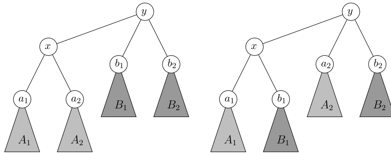
Fig. 2. Replacing quartets in Make-it-Connected.
