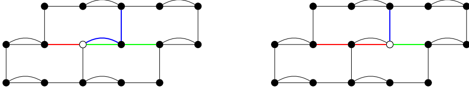
Figure 3: Swapping branch vertices.
