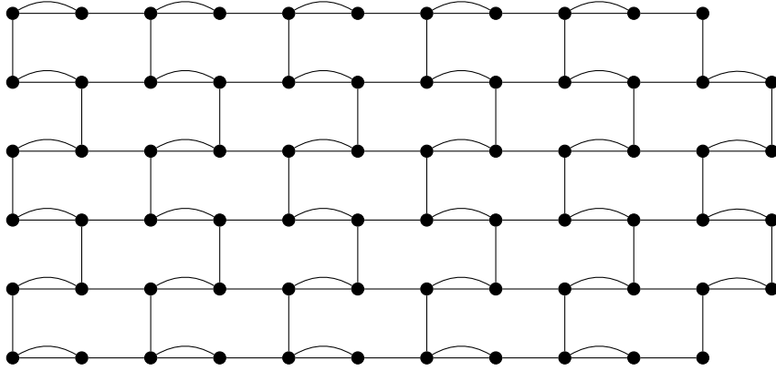
Figure 1: The graph \widehat{W}_5 .
