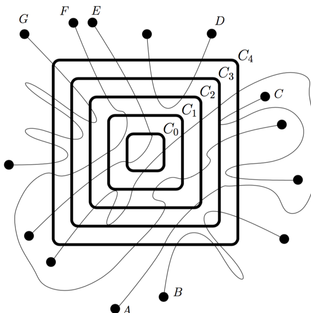
Figure 3: An example of a CL-configuration \mathcal{Q} = (\mathcal{C}, L) where \mathcal{C} contains 5 cycles and L has 7 paths. \mathcal{Q} has 13 segments. Linkage paths A , B , C , D , E , F , and G , contain 2, 2, 2, 1, 1, 2, 3 of these segments respectively. Also the eccentricities of the segments of A , are 0 and 2, of B are 3 and 4. Notice that one of the two segments of A has two 3-chords, each having 2 semi 3-chords.
