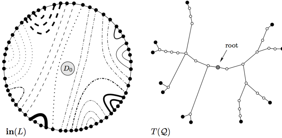
Figure 9: The graph \text{in}_{D_r}(L) for some convex CL-configuration \mathcal{Q} = (\mathcal{C}, L) and the tree T(\mathcal{Q}) . Internal edges in \text{in}_{D_r}(L) of the same type are drawn as lines of the same type. \mathcal{Q} has 11 extremal segments, as many as the leaves of T(\mathcal{Q}) . The relation \parallel has 19 equivalent classes. The dilation of T(\mathcal{Q}) is 4, its height is 8 and its real height is 4.
