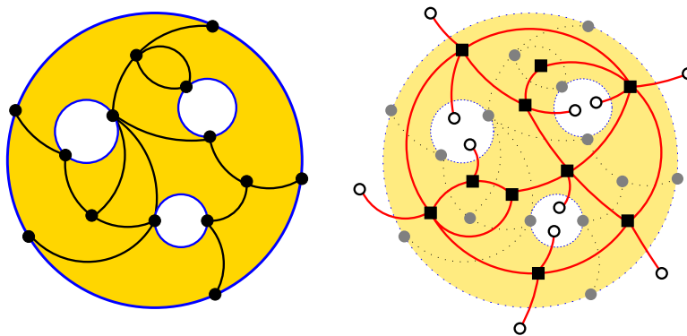
Fig. 1. A map with boundary and its dual.
