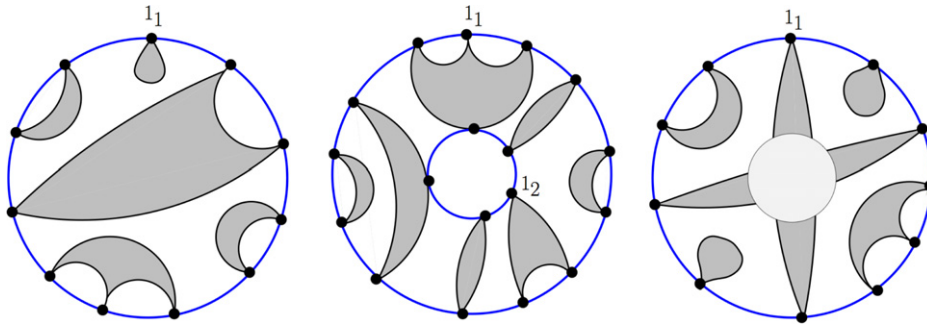
Fig. 2. Geometric representation of non-crossing partitions on a disk, on a cylinder, and on a Möbius band. (For interpretation of the references to colour in this figure legend, the reader is referred to the web version of this article.)
