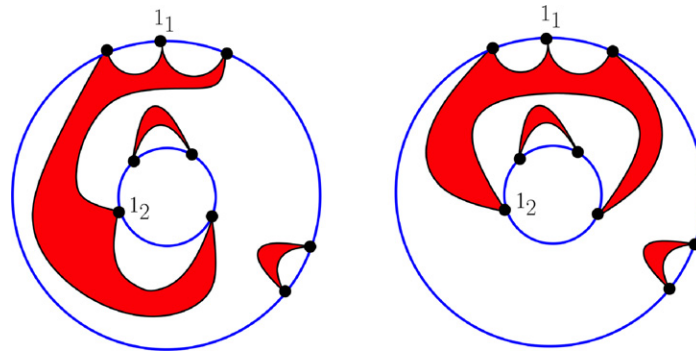
Fig. 10. Two different representations of the same partition.
