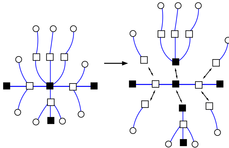
Fig. 7. A double tree and its decomposition.
