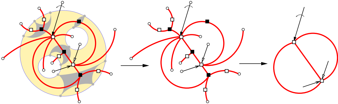
Fig. 8. The construction of the scheme of an element in \mathcal{P}_\Sigma . We consider the dual of an irreducible bipartite subdivision (leftmost figure). After deleting vertices of degree one recursively and dissolving vertices of degree two, we obtain the associated scheme (rightmost figure). (For interpretation of the references to colour in this figure legend, the reader is referred to the web version of this article.)
