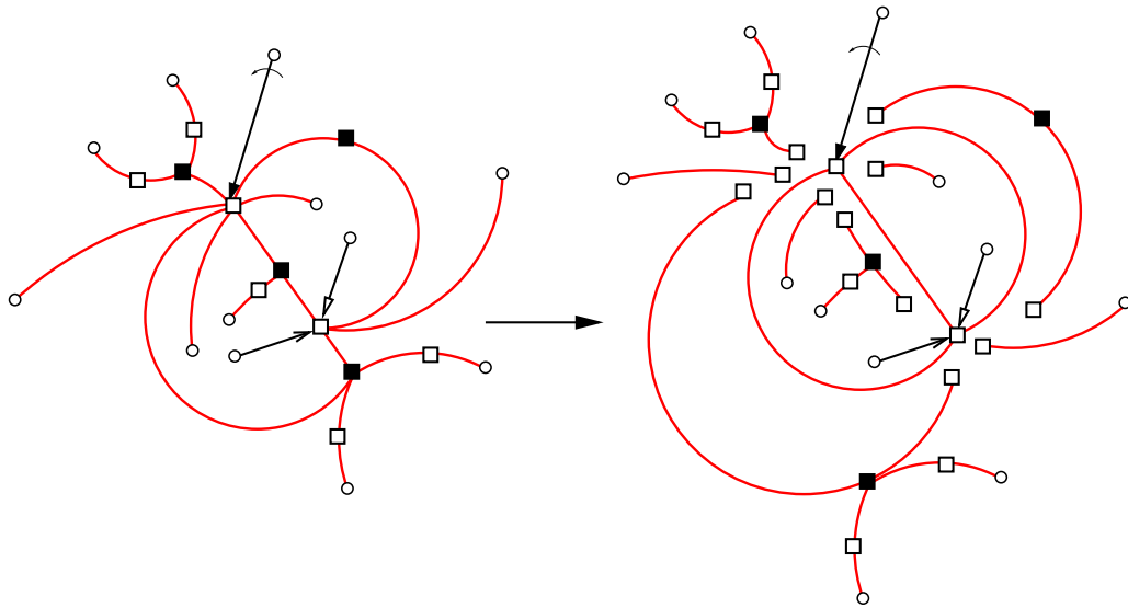
Fig. 9. The decomposition into bicolored trees and the associated scheme. (For interpretation of the references to colour in this figure legend, the reader is referred to the web version of this article.)
