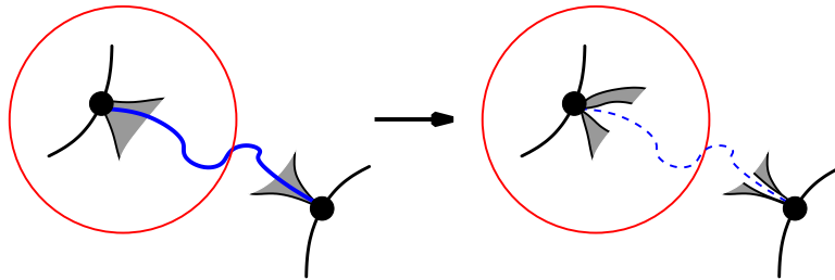
Fig. 5. The operation of joining boundaries.
