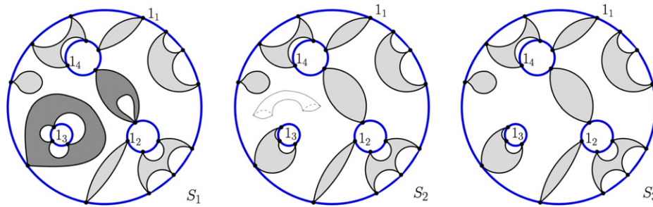
Fig. 3. Three bipartite subdivisions S_1 , S_2 , and S_3 . S_2 is regular but not irreducible, while S_3 is irreducible.
