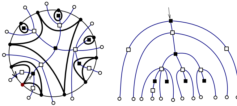
Fig. 6. A non-crossing partition on a disk and the associated tree.
