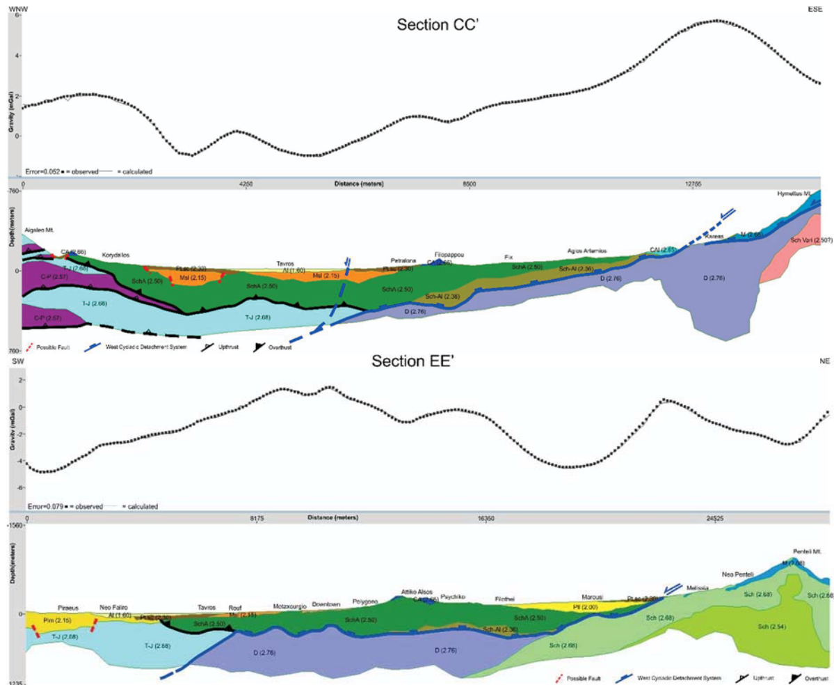
Figure 2. Interpretative geological 2.75-D profiles (scale 1:2). The observed (squares) and calculated (line) residual anomaly are illustrated. The geological formations are: T-J: Triassic-Jurassic Limestones (Ypopelagoniki Unit), C-P: Shales and Sandstones alterations (Ypopelagoniki Unit), M: Marbles (Metamorphic Unit), Sch: Schists (Metamorphic Unit), D: Dolomites (Metamorphic Unit), Sch-Vari: Varis Schists (Metamorphic Unit), SchA: Athens Schists (Athens Unit); CA: Limestones (Athens Unit), Sch-Al: Schists (Alepovouni Unit), CAL: Limestones (Alepovouni Unit), Msl: Upper Miocene Terrestrial and Lacustrine deposits (Neogene Formations), Pt.sc: Pleistocene Talus and Screes, Al: Alluvium deposits (Loose Quaternary deposits).
