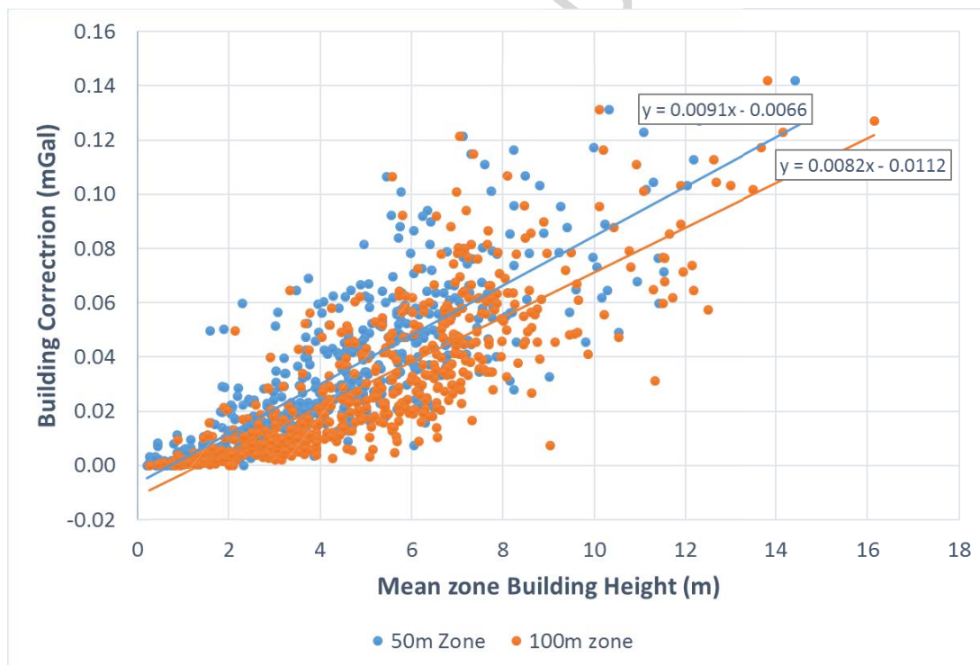
Fig.12. Correlation of mean Building Height with the respective calculated Building Correction. The blue dots refer to the 50 meters radius zone and the red for the 100 meters radius zone.
