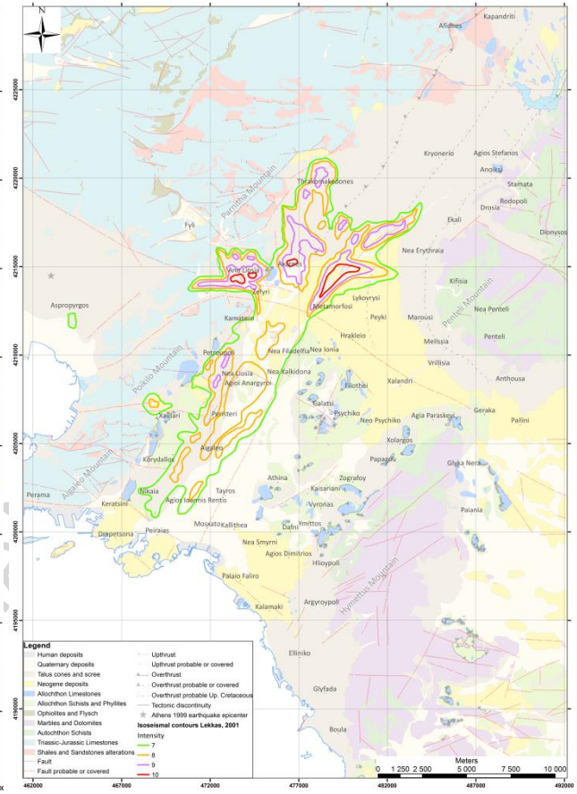
Fig.3. Isoseismal contours by Lekkas E. (2001)
