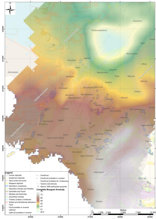
Fig.5. Complete Bouguer Anomaly map
