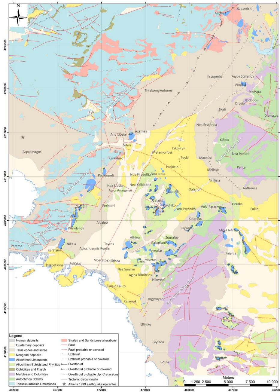
Fig.1. Geologic and tectonic regime of Athens basin, along with the Athens earthquake of 7 th September 1999.
