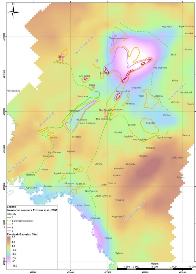
Fig.7. Residual Anomaly map and Isoseismal contours by Tzitziras et al. (2000).
