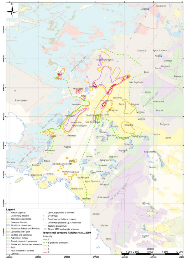
Fig.2. Isoseismal contours by Tzitziras et al. (2000)
