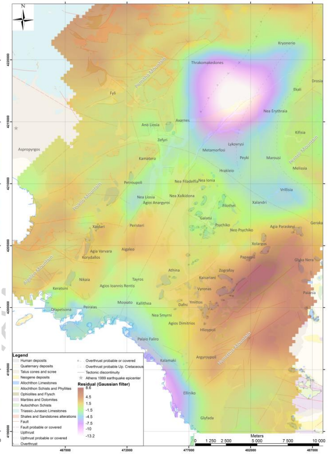
Fig.6. Residual Anomaly map
