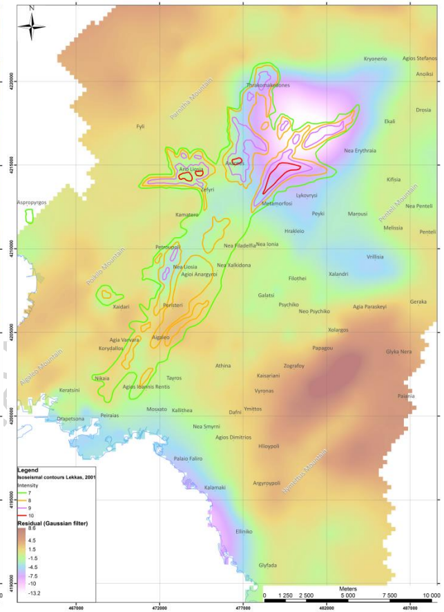
Fig.8. Residual Anomaly map and Isoseismal contours by Lekkas E. (2001).
