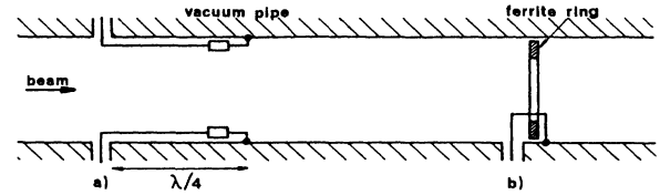
FIG. 9. Loop-type and ferrite ring-type pick-ups (or kickers). Note that for loop-type kickers the beam direction should be inverted.
