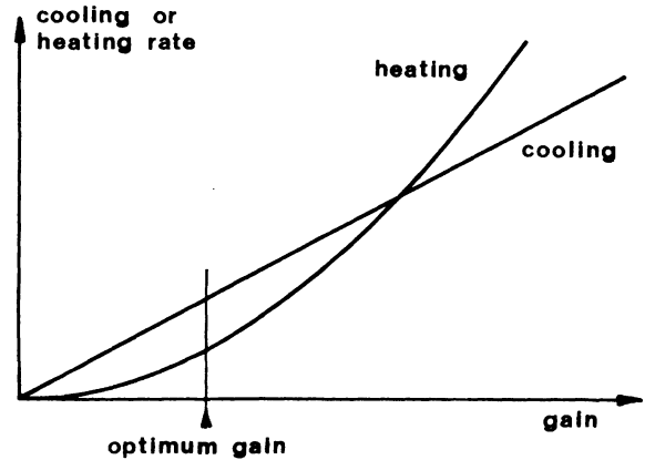
FIG. 3. Variation with system gain of the coherent cooling and incoherent heating effect.
