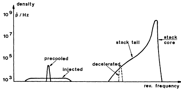
FIG. 11. Density distribution vs revolution frequency in the Antiproton Accumulator. On the right, the stack; on the left, the newly injected batch, before and after precooling.
