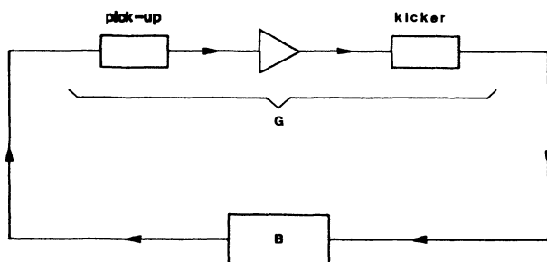
FIG. 6. Beam feedback effect. The loop is closed by the coherent beam response B .
