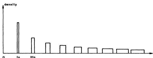
FIG. 5. Longitudinal Schottky bands originating from a large group of particles with slightly different revolution frequencies. At high frequencies the bands overlap.
