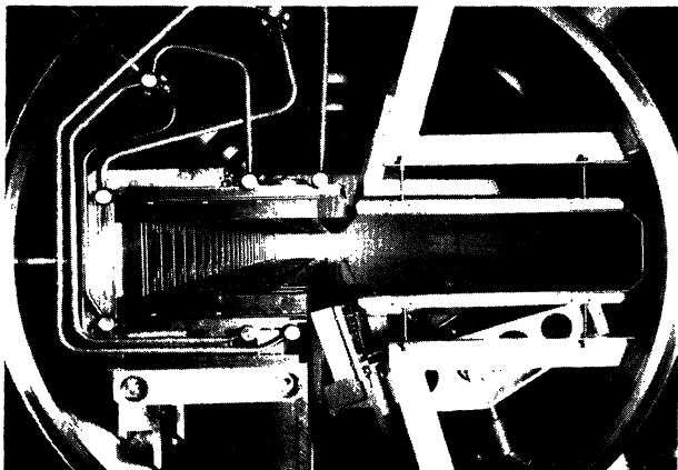
FIG. 12. Inside of a vacuum tank with precooling kickers at the left and space for the stack at the right. The ferrite frames of the kickers are open in the centre of the picture; they can be closed by the ferrite slabs mounted on the shutter that rotates around a pivot at the far right. Water tubes for cooling the ferrite may be seen.
