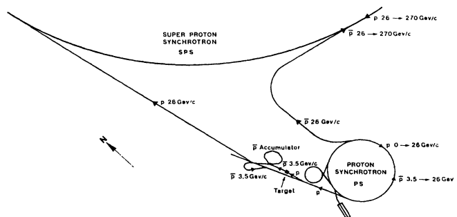
FIG. 1. Overall layout of the p\bar{p} project.
