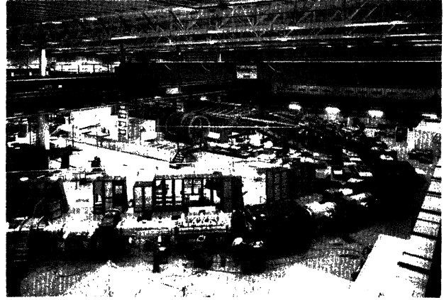
FIG. 15. View of the Antiproton Accumulator before it was covered by concrete slabs. The silvered material around the vacuum tanks is insulation, needed because everything may be heated to 300° to obtain ultrahigh vacuum. The transmission lines crossing the ring and carrying the cooling signals may be seen.
