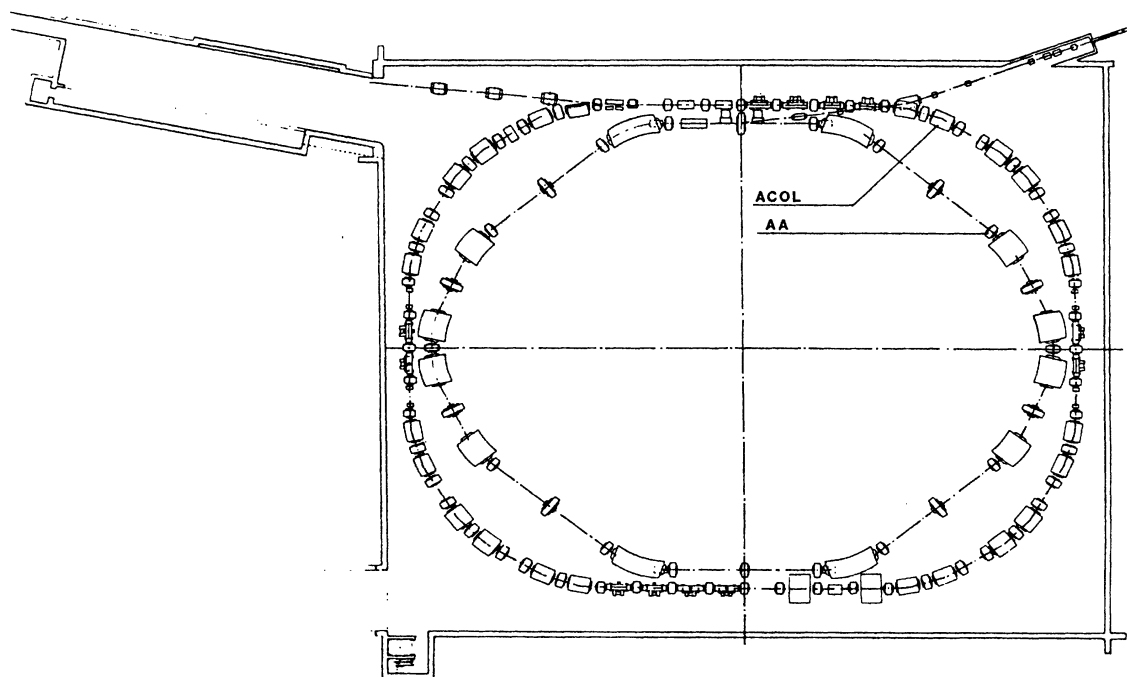
FIG. 16. The new ACOL ring (under construction) around the AA. This ring will increase the stacking rate by an order of magnitude. The stack will still be kept in the AA ring.
