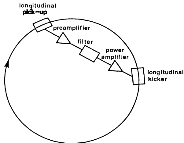
FIG. 7. Filter cooling.
