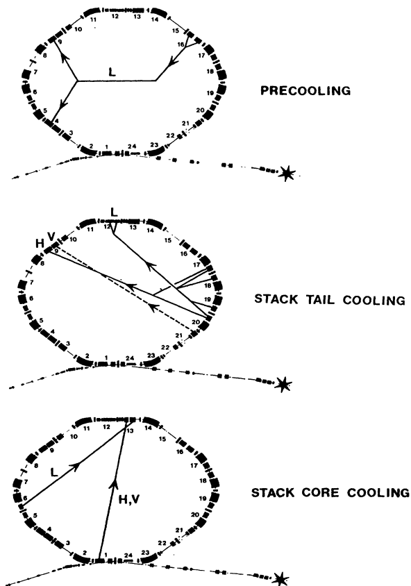
FIG. 14. Plan of the AA ring with its 7 cooling systems. L=longitudinal, V=vertical, H=horizontal.
