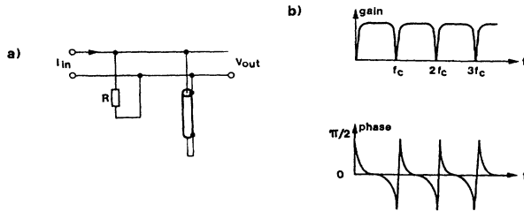
FIG. 8. (a) Simple transmission-line filter. (b) Amplitude and phase response vs frequency.
