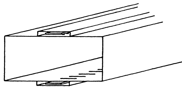
FIG. 10. Slot-type pick-up or kicker. One end of the transmission line is terminated with its own characteristic impedance.
