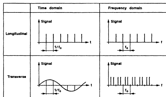
FIG. 4. Schottky signals in time domain and frequency domain.
