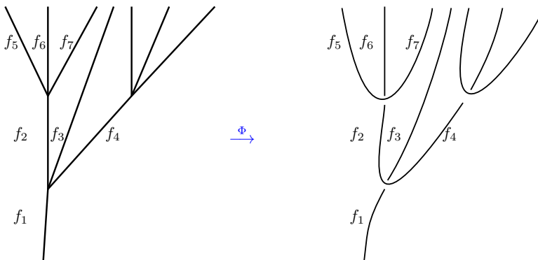
Fig. 8. Relating a forest to a tangle via the functor \Phi .
