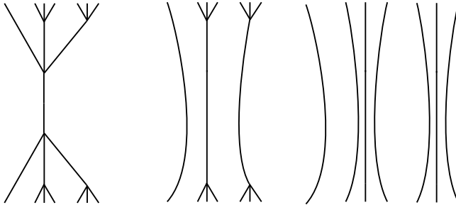
Fig. 3. A series of simplifications in the group multiplication.
