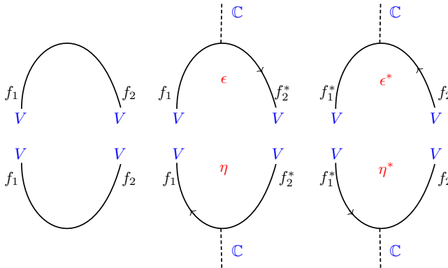
Fig. 5. The cup and cap maps.
