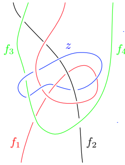
Fig. 4. A decorated (n, m) -tangle.
