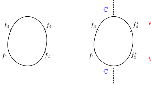
Fig. 7. Composing cup to cap.
