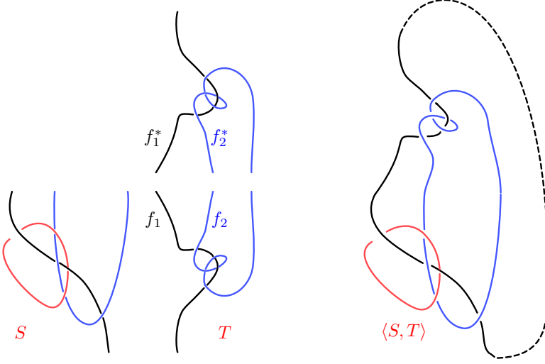
Fig. 9. The inner product of two decorated tangles.
