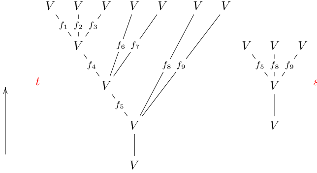
Fig. 1. Two decorated trees; the upward arrow indicates the direction of the maps.
