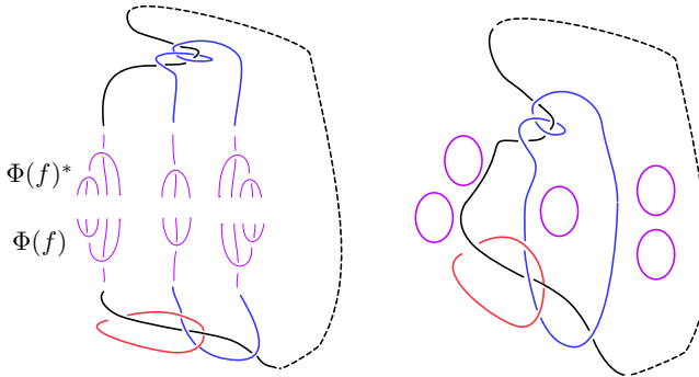
Fig. 11. Canceling carets after composing by the image \Phi(f) of a forest f with 5 nodes.
