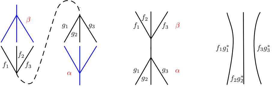
Fig. 2. Multiplying the Thompson group elements \alpha, \beta .
