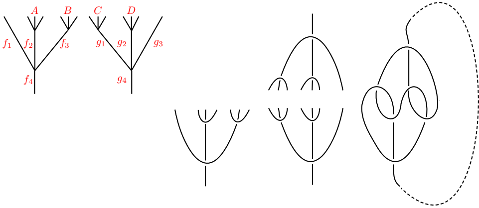
Fig. 12. Computing the inner product of tangles coming from trees.
