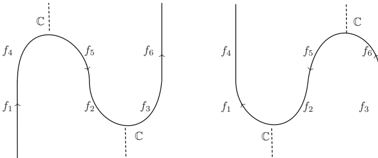
Fig. 6. Composition of maps in a bottom-to-top arc.
