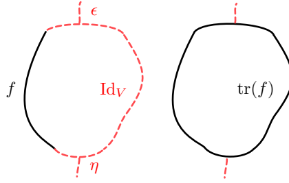
Fig. 10. Closing the bottom-top arc.
