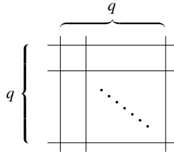
Fig. 3. The analytic reduction of X_{t,c}
