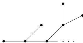
Fig. 1. The mirror of a parabolic element if q = 2
