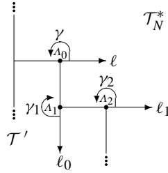
Fig. 2. The infinite sequence \{\ell_i\}
