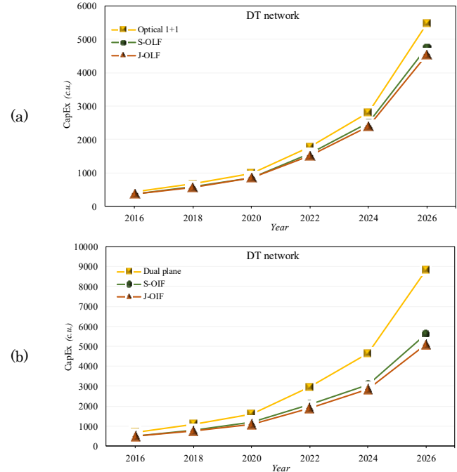
Fig. 7 Capital Expenditure for the DT network: (a) optical layer survivability (b) multi-layer survivability.
