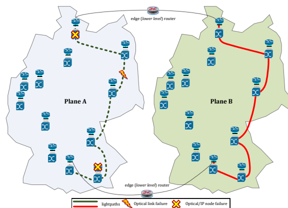
Fig. 2. Dual plane approach: single optical link / (IP & optical) node failure recovery
