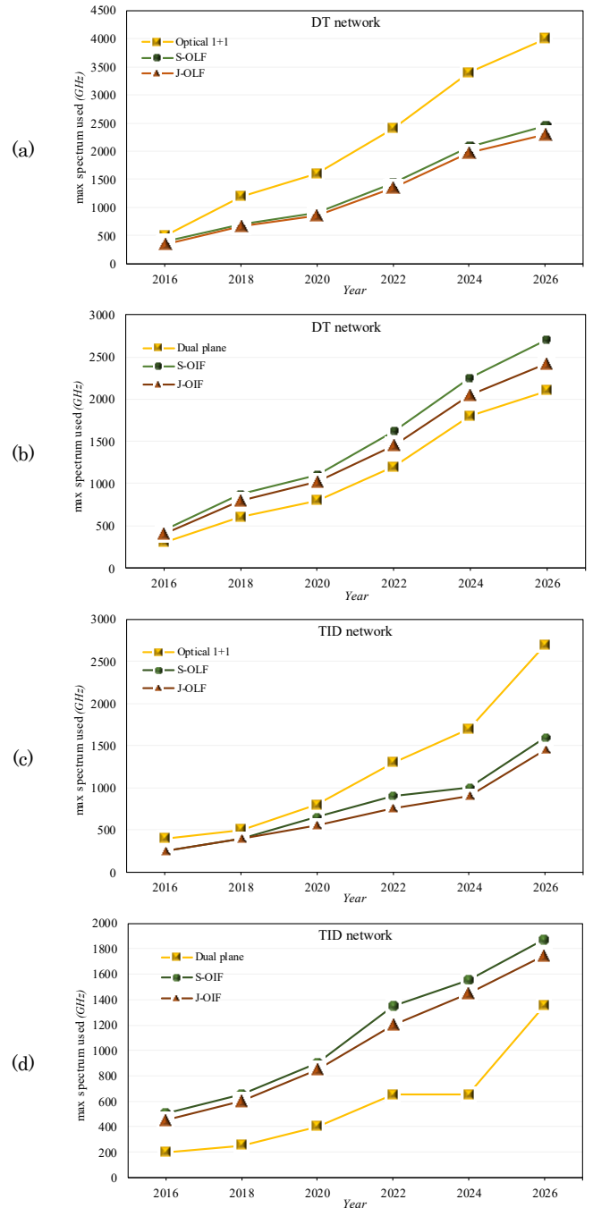
Fig. 9 Maximum spectrum used for the DT network topology: (a) optical layer survivability, (b) multi-layer survivability and Telefónica network topology: (c) optical layer survivability, (d) multi-layer survivability.
