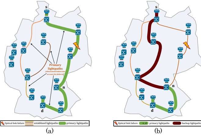
Fig. 4. Integrated multi-layer optical link failure resilience: (a) failure of an optical link along a primary lightpath, (b) setup of the backup path.
