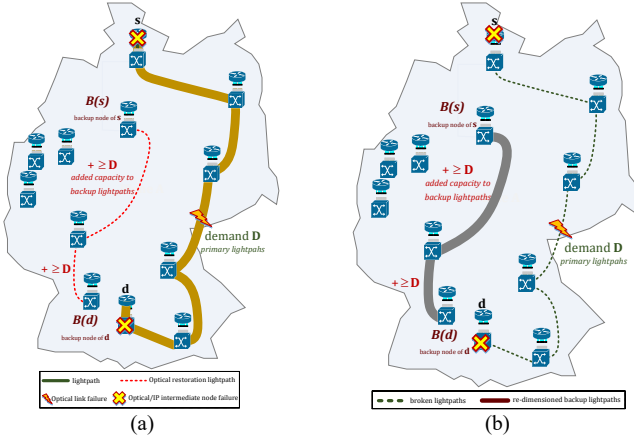
Fig. 5. Sequential multi-layer optical and IP failure resilience: (a) failure (optical link or node failure) along a primary lightpath, (b) setup of the backup path.
