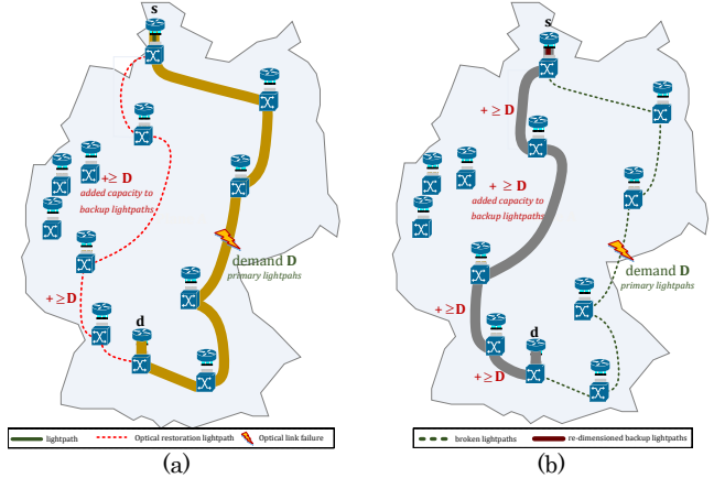
Fig. 3. Sequential multi-layer optical link failure resilience: (a) failure of an optical link along a primary lightpath, (b) setup of the backup path.
