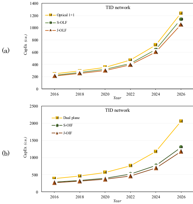
Fig. 8 Capital Expenditure for the Telefónica network: (a) optical layer survivability, (b) multi-layer survivability.
