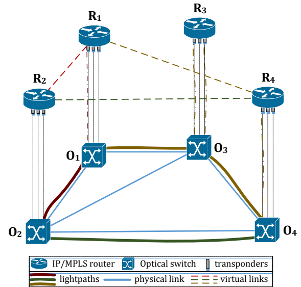
Fig. 1. Architecture of IP over elastic optical network
