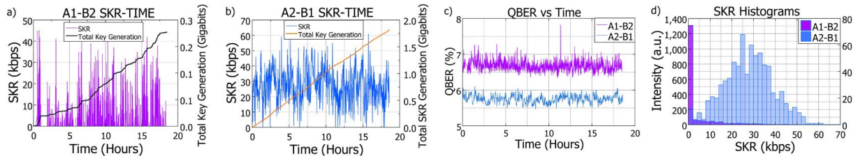
Fig. 3. a) A1-B2 SKR-TIME b) A2-B1 SKR-TIME c) QBER for switched QKD pairs d) SKR Histogram for switched QKD pairs.
