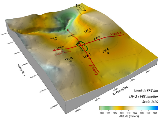
Figure 3a Geophysical locations at “Livadies” pond.
