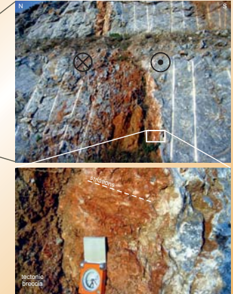
Nevertheless, several dextral strike slip tectonic structures trending WSW-ESE, possibly related to the northern branch of the active North Aegean Trough, can be identified across the marginal range by observing the shaded relief maps. This mountain range is the highest morphological relief between the basin and the trough, the tectonic influence of which seems to affect the range and fade away more westerly in the intra-basin area, as the paleo-relief of the alpine basement extracted by geoelectrical measurements show. The dextral character of these cross cutting structures is clear either by examining the subsurface basement map or by observing the drainage network offset on each side of the morpho-lineaments that can be attributed to strike slip faulting. Additionally, almost horizontal striations on vertical fault surfaces were observed at marble outcrops located at the eastern marginal area, accompanied with kinematic indicators compatible with dextral movement (see photographs above).
