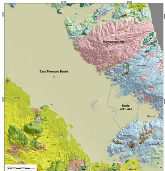
Fig. 2: Simplified geological shaded relief map of the basin and its marginal area. Pale colours refer to Quaternary (1) Pleistocene (2) and Miocene (3) sediments, whilst intense colours refer to the alpine basement rocks, Flysch (4), Limestones (5), Ophiolites (6), Amphibolites (7), Marbles (8), Schistolites (9) and Gneiss (10). The dashed outline shows the borders of the recently filled artificial lake of Karla and west of it several basement rocks are cropping out in the middle of the basin.
