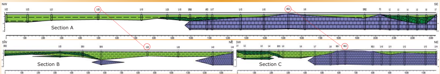
Three litho-stratigraphical sections were composed, based on the interpretation of the resistivity values measured by the VES as well as the borehole stratigraphic data. The section traces are displayed below and note that the vertical scale is exaggerated (x2) for best viewing results.
