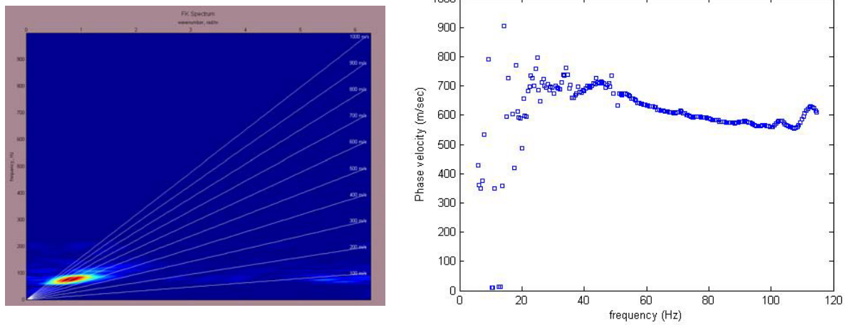
Figure – 5. Characteristic f-k spectrum and dispersion curve (test with 15m distance between source – geophone).
