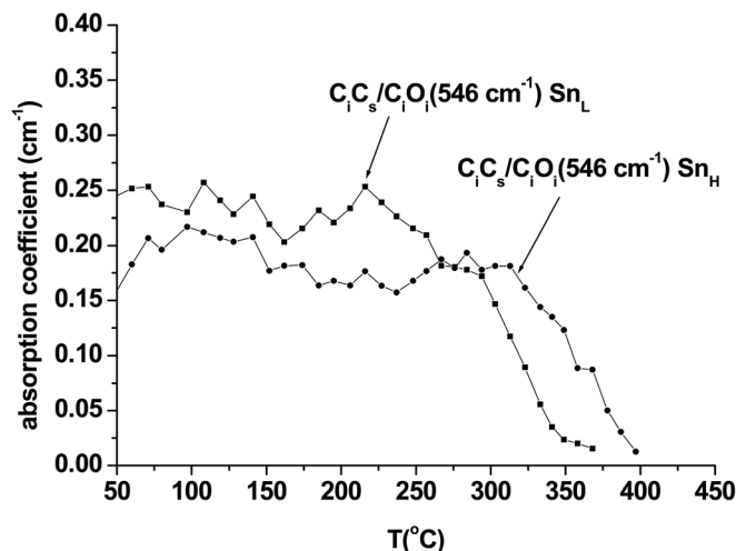
FIG. 6. The thermal evolution of the 546\text{ cm}^{-1} band of the C_iO_i/C_s defects for the Sn_L and Sn_H samples.
