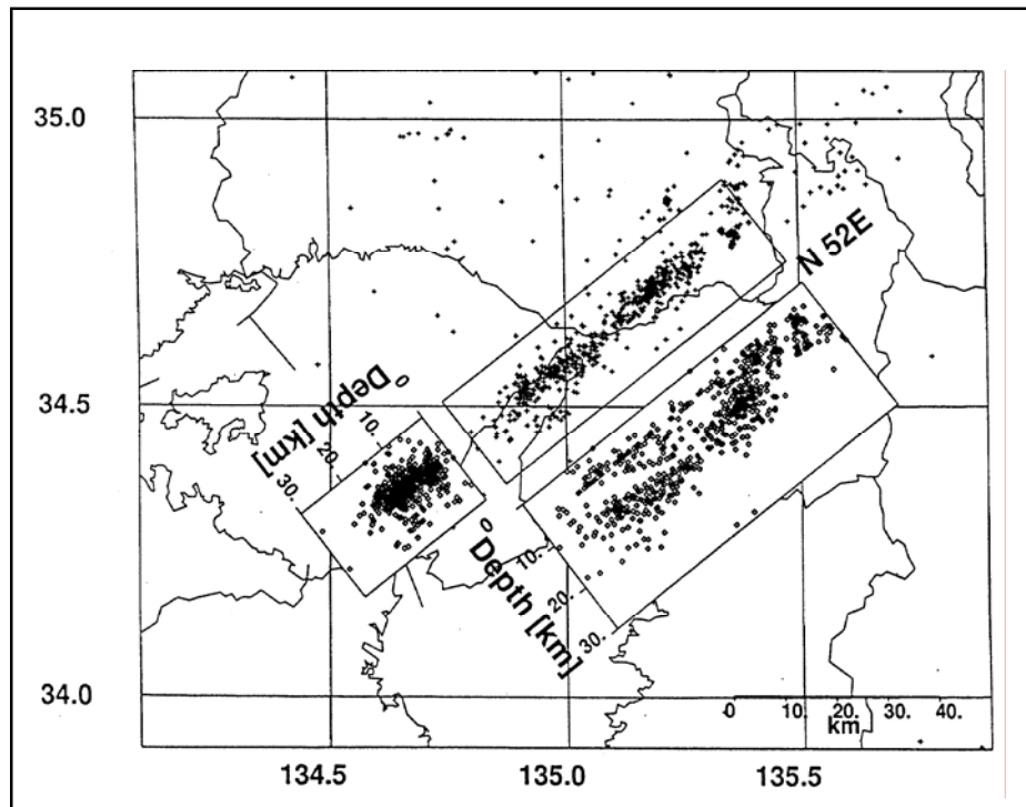
Figure 3. Epicentral distribution of aftershocks.
