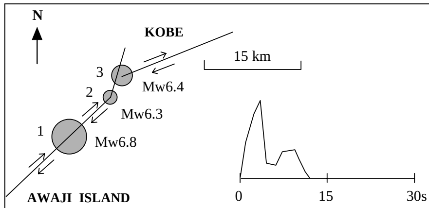
Figure 4. The mechanism of the Hyogo-ken Nanbu earthquake (after Sato et al. [7]).
