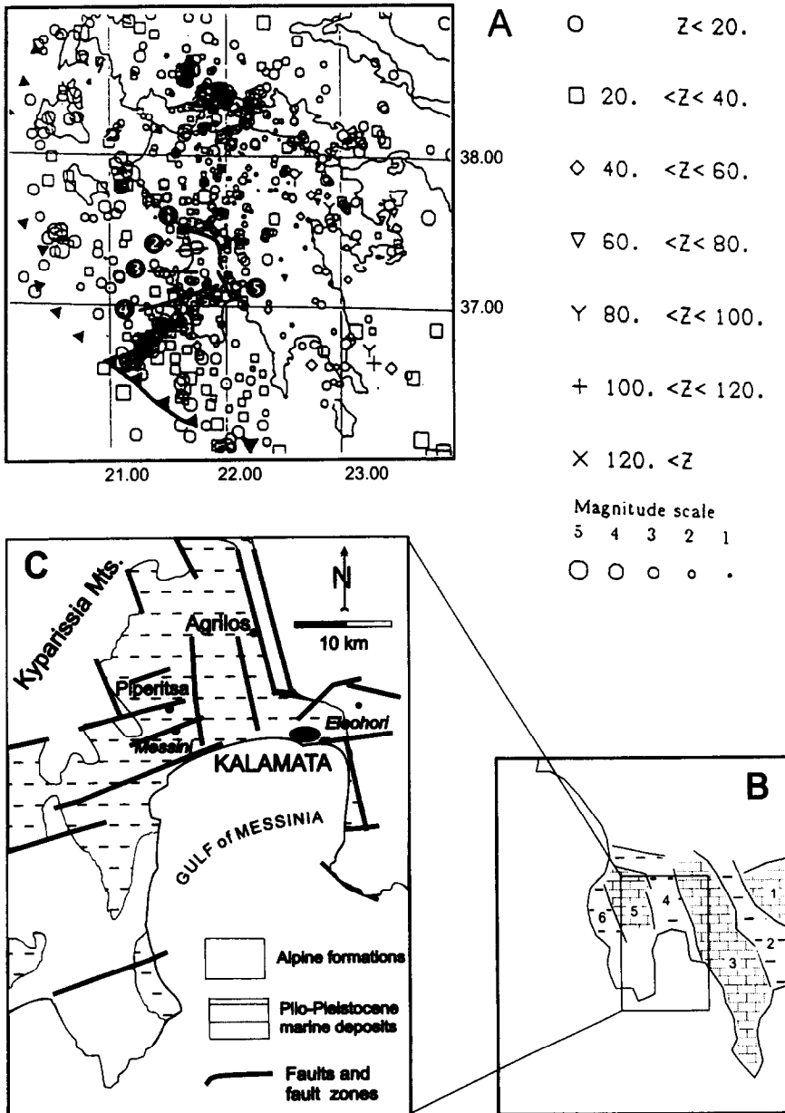
Fig. 1. (A) Earthquake epicentre map of Peloponnessos after Hatzfeld et al. (1990). Numbers in black circles indicate interpreted tectonic lineations by Fountoulis (1994). (B) First-order neotectonic macrostructures of the Southern Peloponnessos. The numbers correspond to the neotectonic macrostructures described in the text. (C) The neotectonic sub-graben of Kato Messinia and its dominant tectonic structures.
