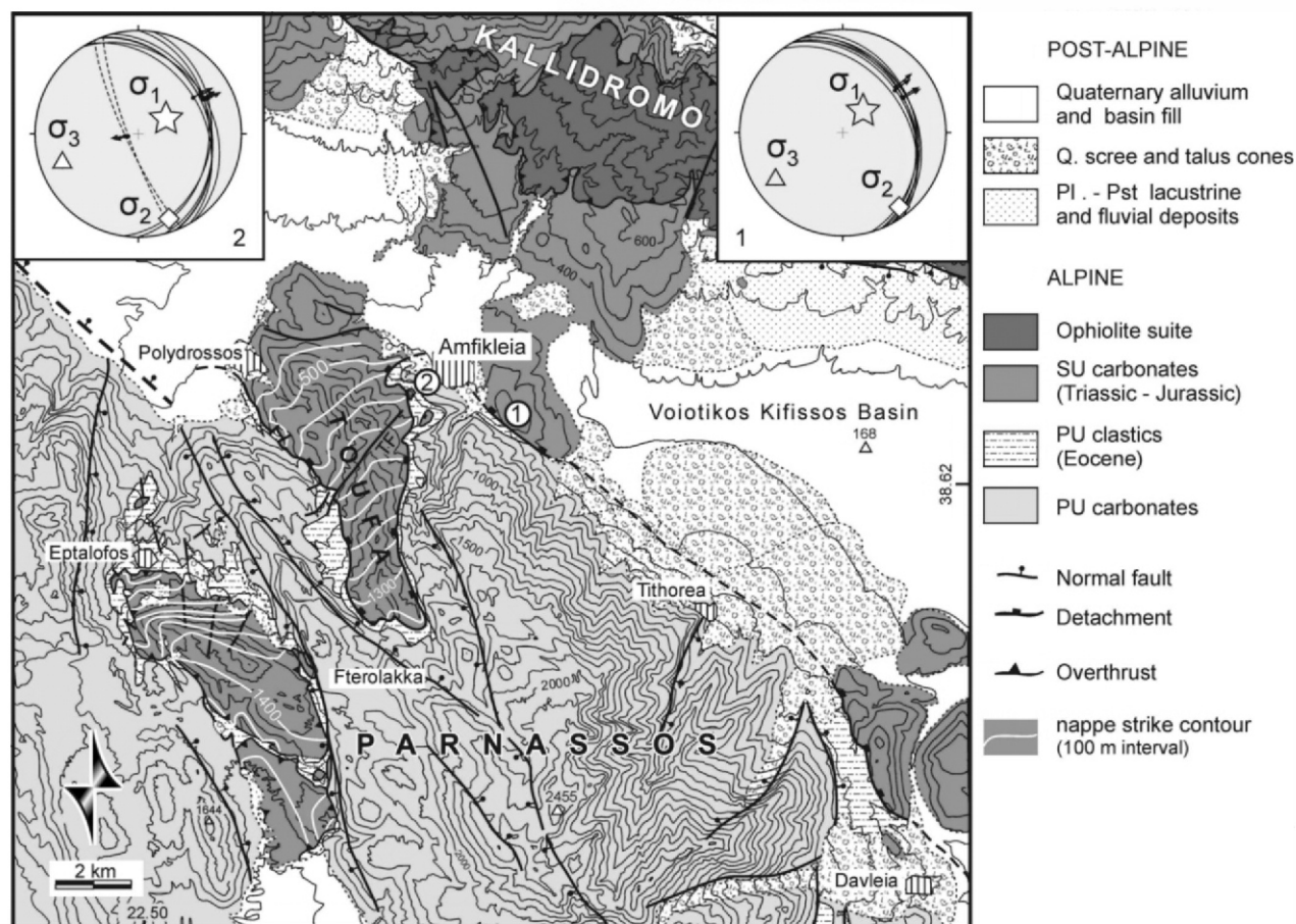
Fig. 2. Tectonic map of Mt Parnassos and environs. Insets 1 & 2 are stereo-plots (equal area, 1. hemisphere) of tectonic data (shear planes) from Dadi hill and Dadi monastery, respectively. Dashed great circles in projection 2 are hangingwall antithetic faults. SU: Sub-Pelagonian Unit; PU: Parnassos Unit.
