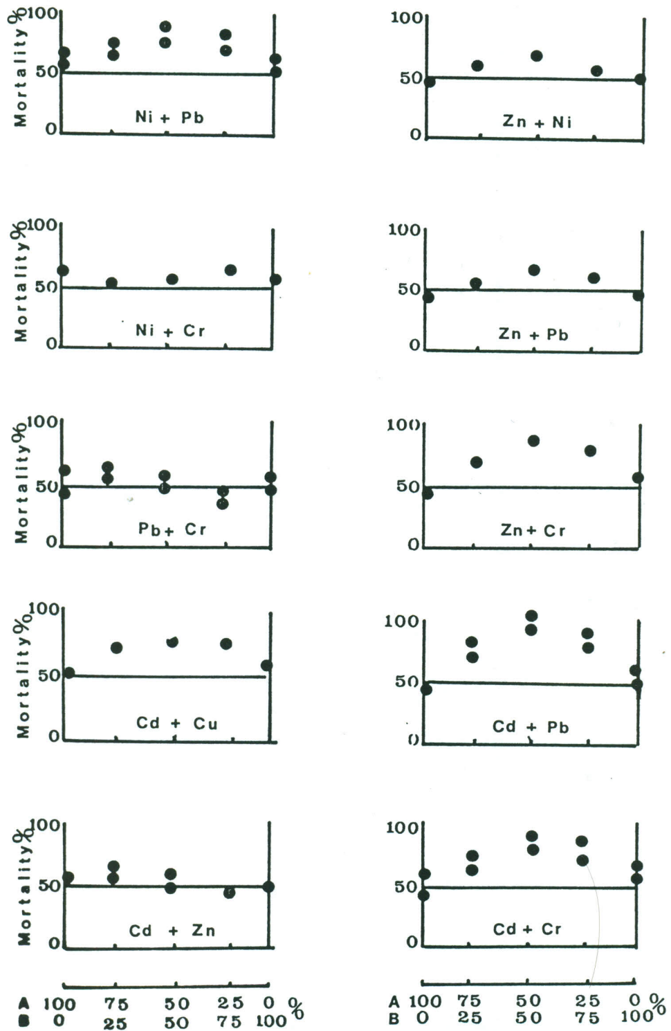
Figure 3. Combined effects of mixtures of two metals (A + B) on the mortality of Tisbe .
