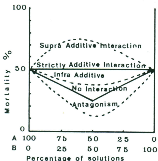
Figure 1. Possible types of responses which can occur between two hypothetical toxicants, A and B, which have similar actions. (Warren 1971).
