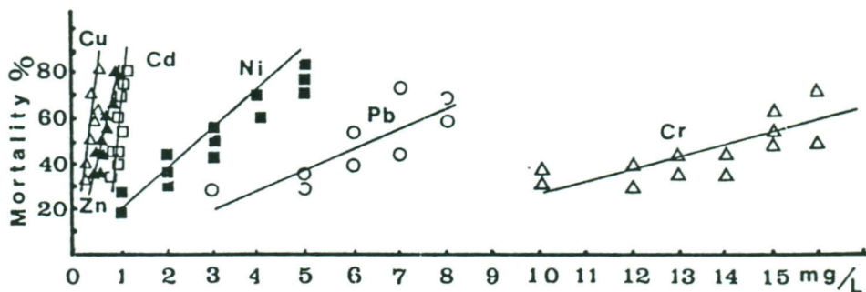
Figure 2. Determination of 48 h LC50 of the different heavy metals according to the Bliss method (1938).
