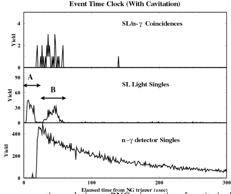
Fig. 3. Event occurrence time relative to PNG trigger time for n/g singles, SL light emission singles, and the SL/n-g coincidences shown with an expanded time scale.
