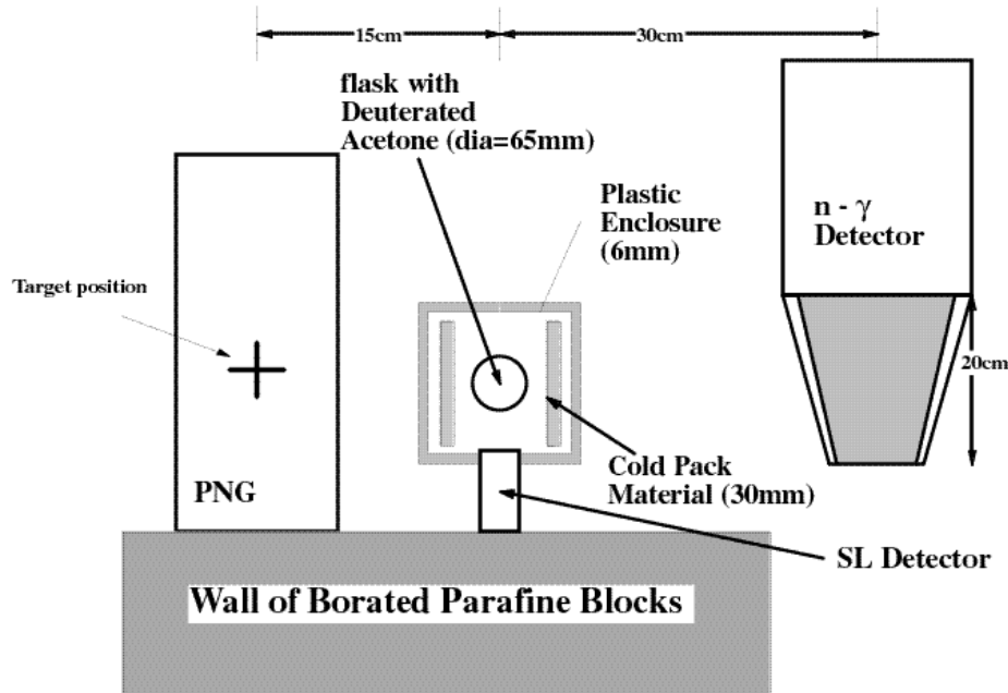
Fig. 1. A rough outline of the detector and shielding arrangement used in the experiment.
