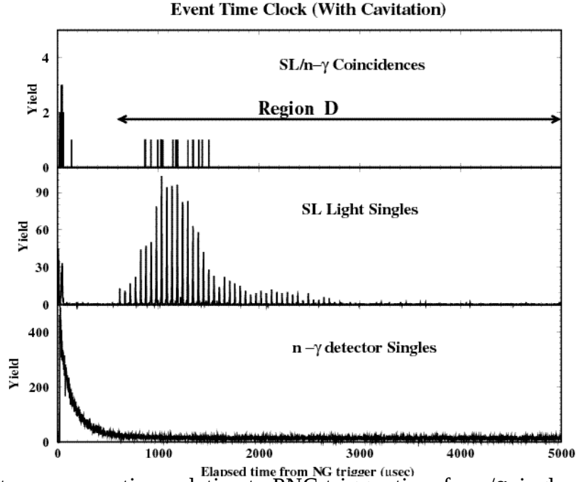
Fig. 2. Event occurrence time relative to PNG trigger time for n/g singles, SL light emission singles, and the SL/n-g coincidences.
