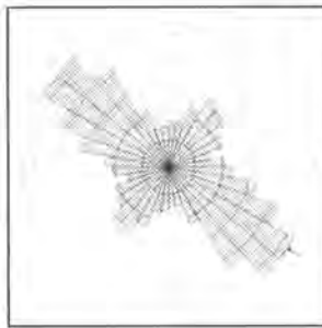
Figure 33. Fractures Rose Plot.
