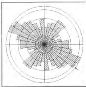
Figure 32. Faults Rose Plot.
