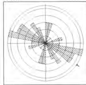
Figure 37. Faults Rose Plot in Granites.
