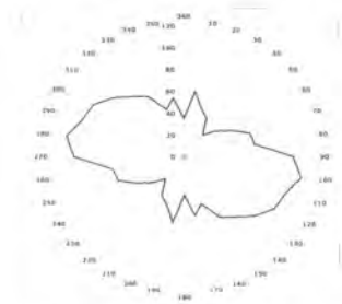
Figure 25. Faults Rose Plot in Cyclades area.
