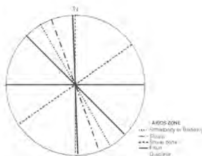
Figure 4. Rose diagram of tectonic elements.
