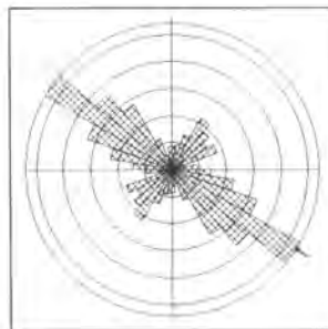
Figure 38. Lineaments Rose Plot in Granites.
