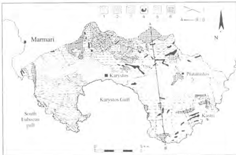
Figure 21. Geology of the study area 2: 1. Alluvium, 2. Marbles and Cipolines, 3. Schists 4. Quartz schists 5. Orthogneisses and 6. Metamorphic basic rocks, 7. Faults.
