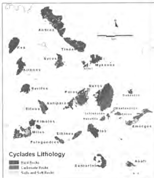
Figure 23. Geographical distribution of the main lithological units at Cyclades area
