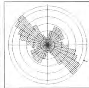
Figure 40. Lineaments Rose Plot Lower Unit.
