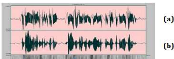
Figure 5. Synchronized signals from the electroglottogram (EGG)(a) and the sound pressure (b).
