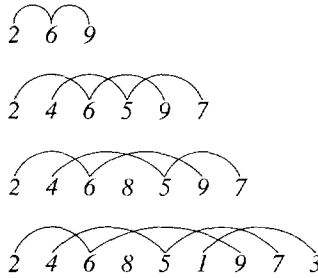
Fig. 3. Constructing the region \sigma_n^{-1}(f) .
