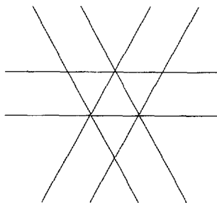
Fig. 1. The Shi arrangement for n=3 .
