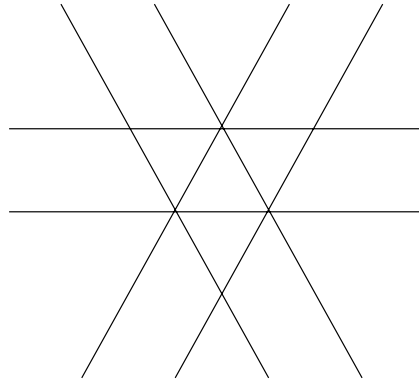
Fig. 2. The Shi arrangement for A_2 .
