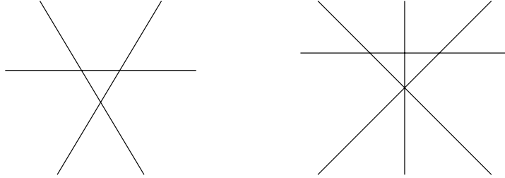
Fig. 3. The Linial arrangements for A_2 and B_2 .
