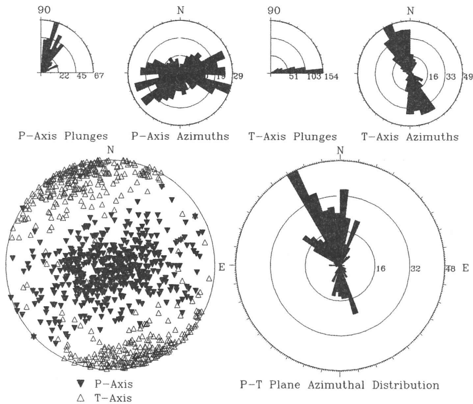
Figure 3. Summary of the seismotectonic features of the Kozani-Grevena aftershock sequence in the form of P and T principal stress axes statistics.
