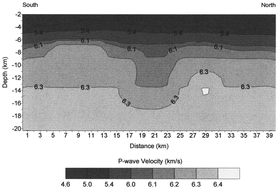
Figure 4. Preliminary results of tomographic inversion in a N-S direction through Paleochori. The low velocity zone at depths of 10-15km is comparable to the focal depth of the main shock.
