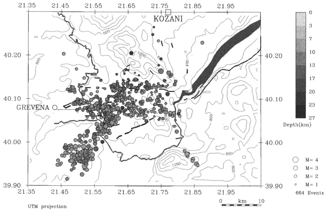
Figure 2. Distribution of the aftershock sequence epicenters, 19-25 May 1995. The dashed line indicates the surface rupture attributed to the main shock.
