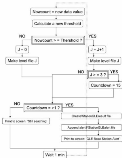
Fig. 3: Flowchart of the Alert algorithm
