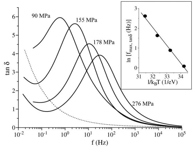
Fig. 1. Isotherms (349 K) of \tan \delta vs frequency of hydrated leucolite. The dash line is a typical measurement on an as-received (not hydrated) specimen at 178 MPa. In the inset diagram, \ln f_{\text{max}, \tan \delta} is plotted against 1/k_B T for P = 155 MPa. The straight line fits the data points.
