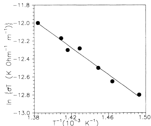
FIG. 3. Conductivity plot obtained from measurements recorded at 5.5 kHz.
