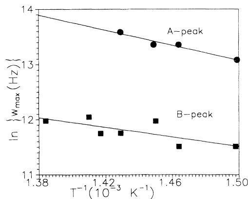
FIG. 2. The temperature dependence of the maxima of the loss peaks.
