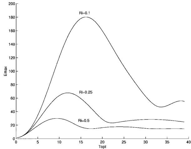
FIG. 10. The optimal energy growth, E_{\max} , as a function of optimizing time T_{\text{opt}} for various Richardson numbers. For larger optimizing times the optimal perturbations assume a roll type structure.
