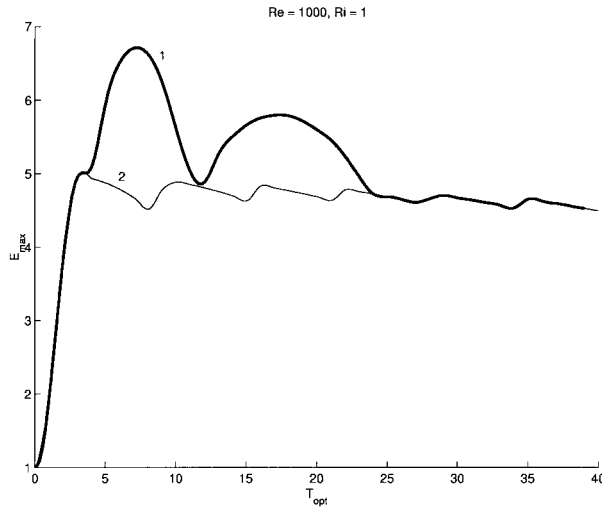
FIG. 15. As in Fig. 13 but for Ri = 1 .
