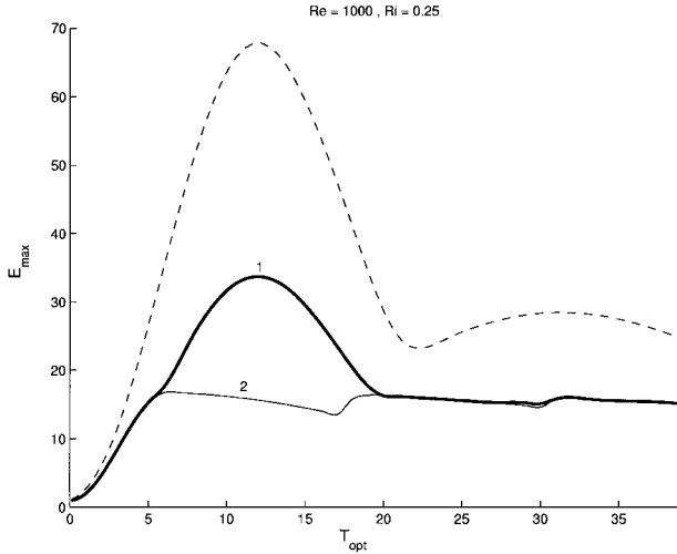
FIG. 13. The optimal energy growth, E_{\max} , as a function of optimizing time T_{\text{opt}} for checkerboard initial perturbations for \text{Ri} = 0.25 and \text{Re} = 1000 . Line 1 (thick solid) shows the energy growth attained by three-dimensional perturbations (for comparison the dashed line shows the growth attained by plane wave perturbations). Line 2 (solid) shows the growth attained by roll perturbations ( k = 0 ). Note that the energy attained by checkerboard initial perturbations is approximately half that attained by the plane wave optimal perturbations.
