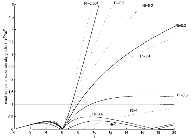
FIG. 3. Evolution of the ratio of the Brunt-Väisälä frequency associated with the perturbation density n^2 = |(g/\rho_m)(\partial\rho/\partial z)| to the Brunt-Väisälä frequency N_0^2 of the background flow for three-dimensional plane wave perturbations with k = 1, l = 6 , and m = 1 (solid lines) and two-dimensional plane perturbations with k = 1, l = 6 , and m = 0 (dashed lines) for various Richardson numbers. The background flow is constant shear unbounded flow and the evolution is inviscid. The initial perturbation energy density has been taken to be 1% of the energy density of the background flow. Whenever the perturbation Brunt-Väisälä frequency exceeds N_0^2 the perturbations may convectively overturn. This may happen very rapidly ( t < 8 ) for perturbations in flows with Ri < 0.4 .
