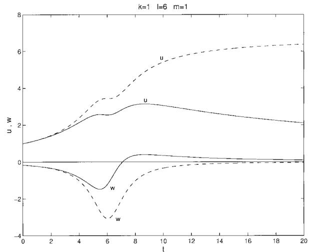
FIG. 2. Evolution of the amplitude of the zonal velocity \hat{u} (dashed line) and vertical velocity \hat{w} (dashed line) for three-dimensional plane wave perturbations with k = 1 , l = 6 , and m = 1 in unstratified inviscid constant shear unbounded flow. The continuous curves show the evolution of the corresponding perturbation velocities in the presence of stratification. The Richardson number is Ri = 0.25 . Note that, as for two-dimensional perturbations, the presence of stratification diminishes the amplitude of the vertical velocity resulting in reduced zonal perturbation velocities. The zonal perturbation velocity does not decay to zero in the inviscid limit but asymptotes to a constant value.
