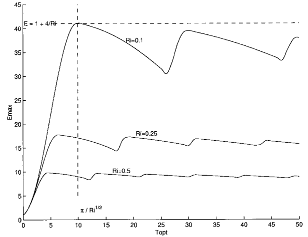
FIG. 6. Optimal energy growth for roll perturbations, E_{\max} , as a function of optimizing time, T_{\text{opt}} , for various Richardson numbers and \text{Re} = 1000 (based on a length scale that makes the nondimensional spanwise wavenumber m = 1 ). Also indicated is the optimal energy growth attained in inviscid flow E_{\max} = 1 + 4/\text{Ri} and the least optimizing time at which it is attained.
