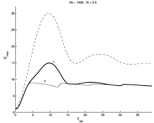
FIG. 14. As in Fig. 13 but for \text{Ri} = 0.5 .
