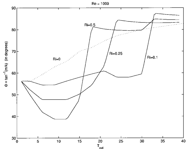
FIG. 9. The degree of obliqueness of the plane wave optimal perturbation as a function of the optimizing time T_{\text{opt}} for various Richardson numbers. The Reynolds number is 1000. The degree of obliqueness is measured by the angle \Theta = \tan^{-1}(m/k) , which measures the angle between normal and the phase lines of the plane wave and the zonal direction. When \Theta = \pi/2 the phase lines are aligned with the zonal direction and the perturbation has roll structure ( k = 0 ). When \Theta = 0 the plane wave is confined in the vertical plane and we have two-dimensional perturbations ( m = 0 ). Note that as the Richardson number increases the optimal perturbations get aligned more to the vertical plane. As the optimizing time increases the perturbations increasingly assume a roll type orientation.
