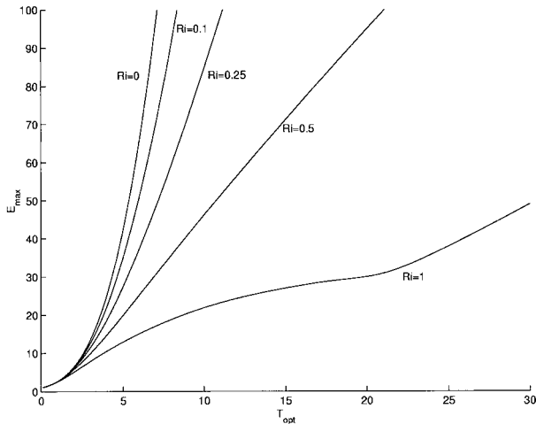
FIG. 8. The optimal energy growth, E_{\max} , as a function of optimizing time T_{\text{opt}} for various Richardson numbers. The flow is inviscid. The growth attained for high Richardson numbers is approximately equal to the square root of the growth attained in the unstratified case ( Ri = 0 ).
