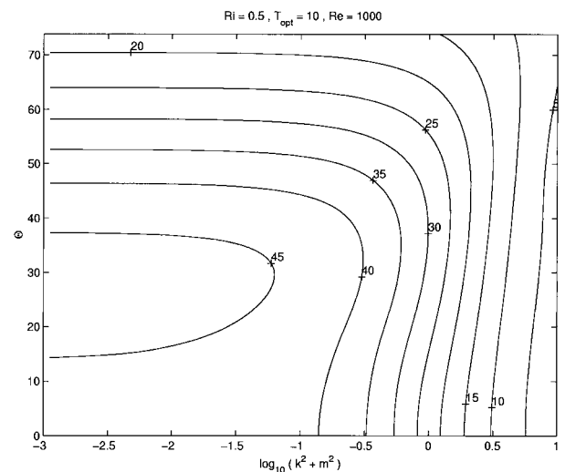
FIG. 12. Same as in Fig. 11 but for Richardson number \text{Ri} = 0.5 . The maximal growth occurs for perturbations with \Theta \approx 30^\circ . The increased stratification has reduced the angle of obliqueness \Theta . For higher Richardson numbers the maximum occurs for lower values of \Theta ; i.e., for \text{Ri} = 0.75 , \Theta \approx 8^\circ , while for \text{Ri} = 1 , \Theta = 0^\circ .
