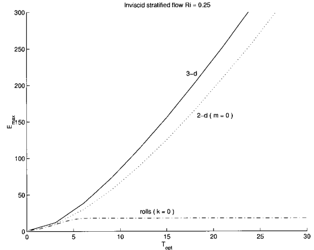
FIG. 7. The optimal energy growth, E_{\text{max}} , as a function of optimizing time T_{\text{opt}} for three-dimensional plane wave perturbations ( m = 0 , solid line), two-dimensional plane wave perturbations ( m = 0 , dashed line), and roll perturbations ( k = 0 , dash-dot line). The Richardson number is \text{Ri} = 0.25 . The flow is inviscid.
