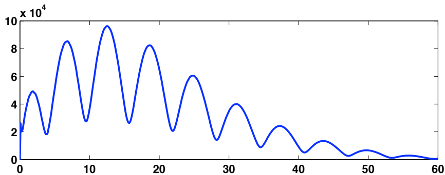
Fig. 5 \|e^{tA}\| , the hump for the stabilized Boeing 767
