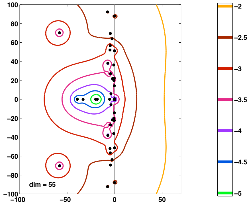
Fig. 6 \epsilon -pseudospectra for the stabilized Boeing 767
