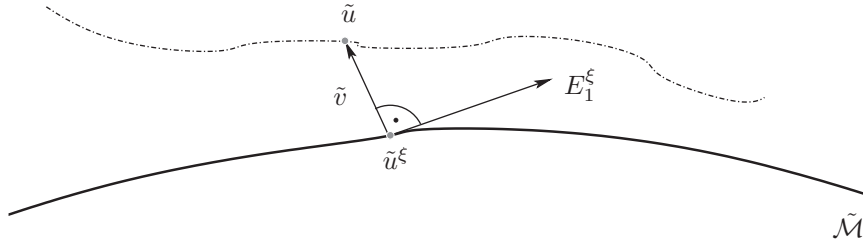
FIG. 1.2. The local coordinate system \tilde{u} = \tilde{u}^\xi + \tilde{v} around \tilde{\mathcal{M}} for N = 1 (two interfaces). Note that E_1^\xi \approx \tilde{u}_1^\xi , which is the tangential vector along the manifold.
