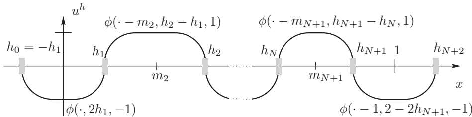
FIG. 1.1. Gluing together positive and negative solutions of (1.3) to obtain u^h \in \mathcal{M} . Note that m_1 = 0, m_{N+2} = 1 , and I_j = [m_j, m_{j+1}] .
