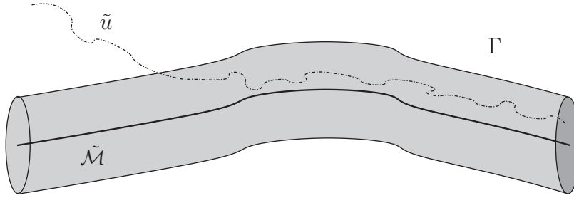
FIG. 2.1. The stability of the slow manifold \tilde{\mathcal{M}} for two interfaces ( N = 1 ). A small tubular neighborhood \Gamma , the slow channel, is attracting over long time scales. Solutions tend to exit at the end of \Gamma by a breakdown of an interface.
